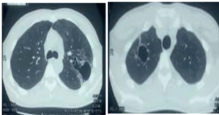
Figure 3. Control thoracic CT on D14 not injected in axial slice, parenchymal window. Resolution of the initial frosted-glass parenchymal lesions and nodular lesions (a) with the appearance of sparse sequellar-looking cavities in the lung parenchyma (b and c).
